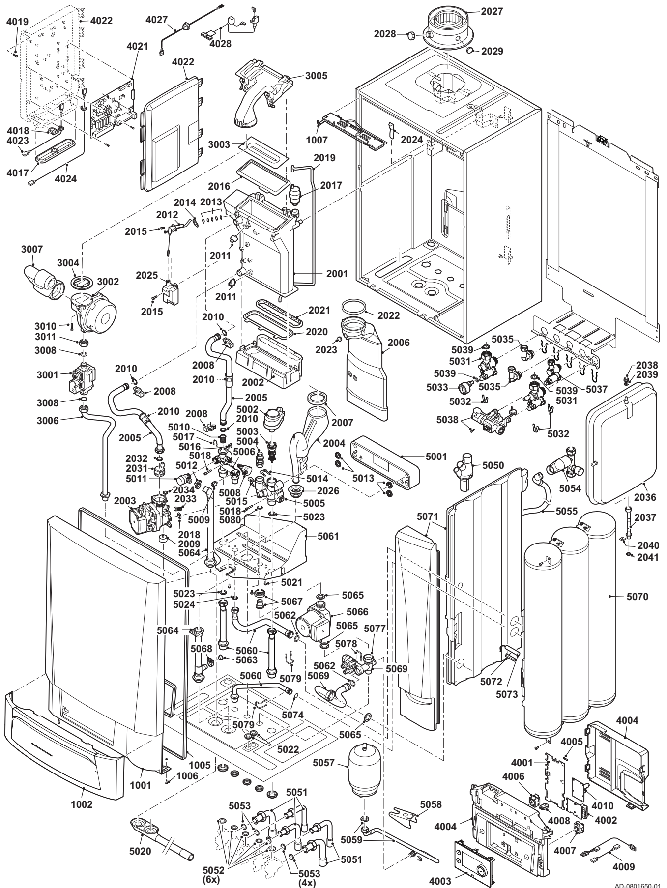
Abb.120 AMC 24/28 BIC
