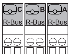
Abb.44 R-Bus-Anschlüsse
