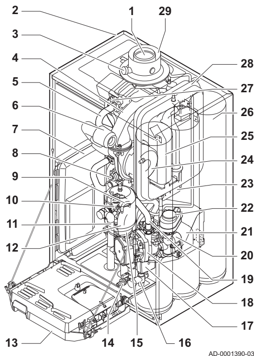
Abb.5 AMC 24/28 BIC
