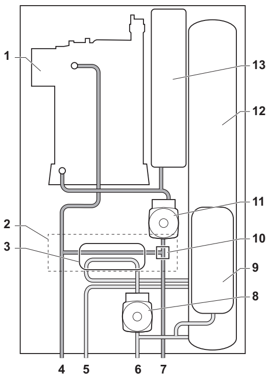
Abb.4 AMC 24/28 BIC
