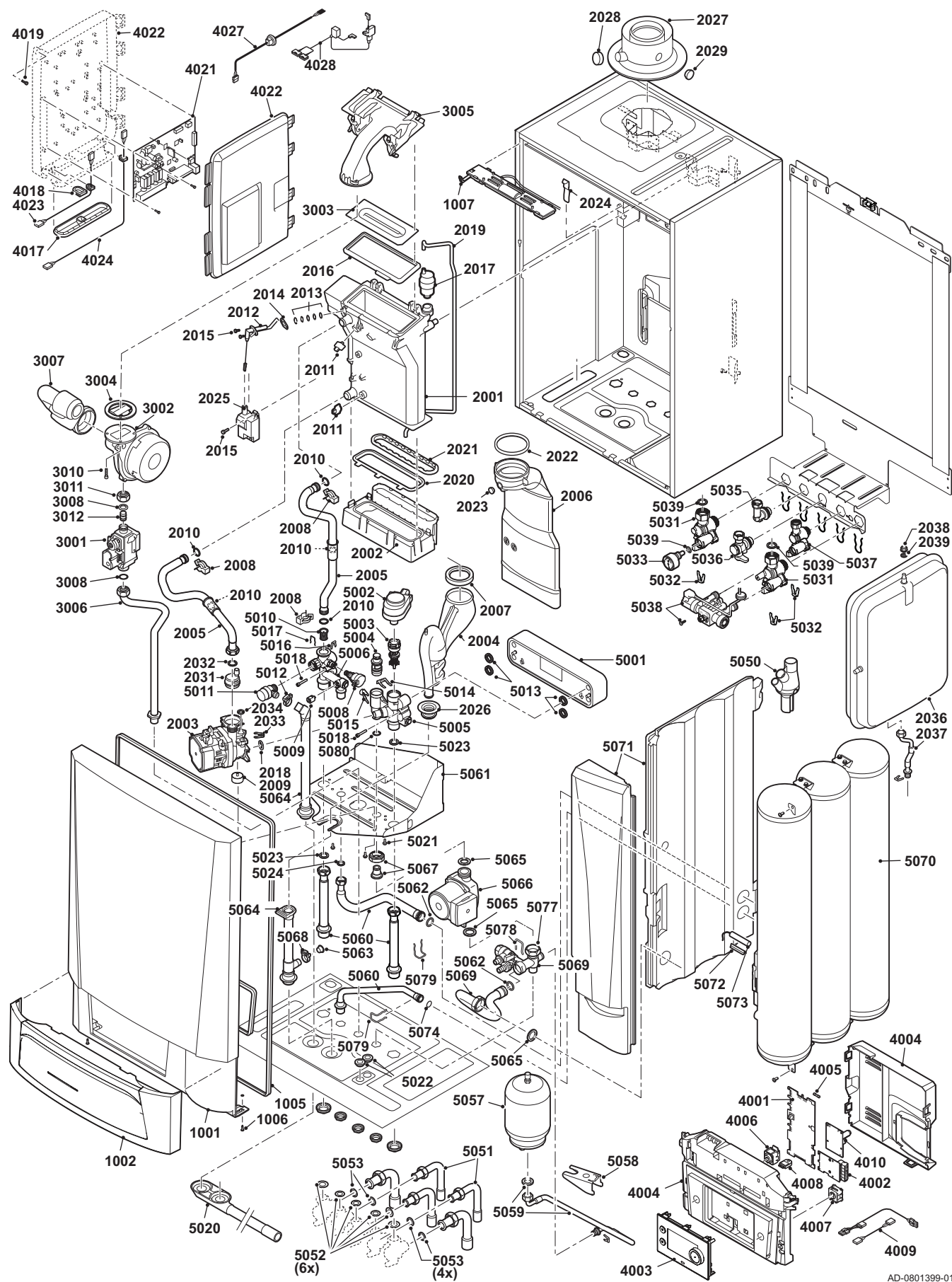
Abb.121 AMC 24/28 BIC
