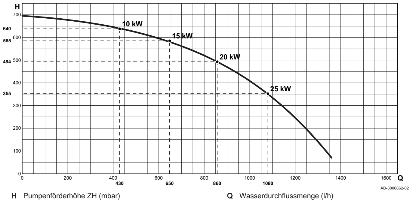
Abb.3 AMC 24/28 BIC
